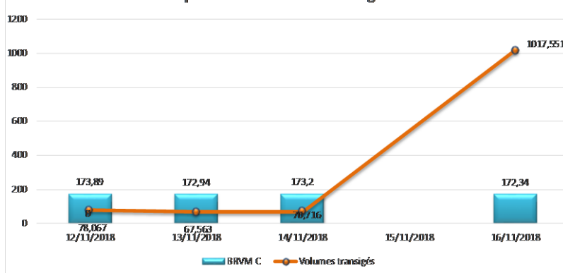
BRVM Composite vs Volumes Transigés
